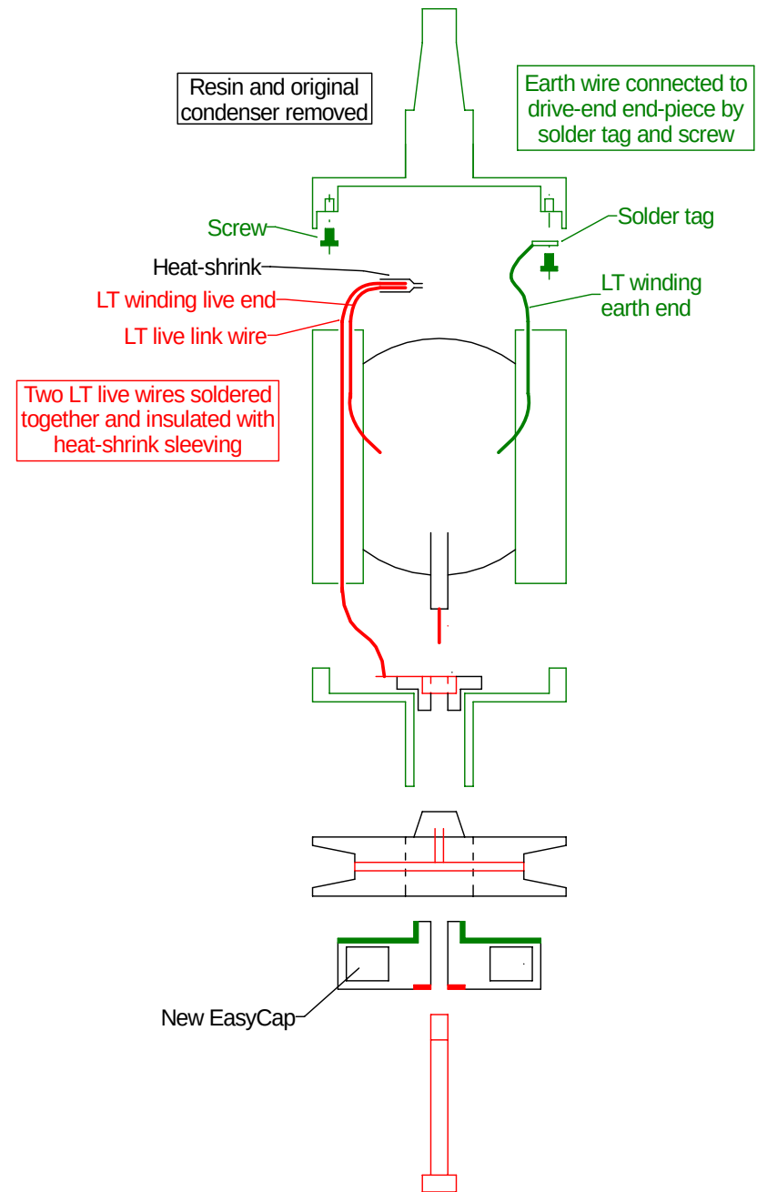
Exploded schematic 'AFTER'
