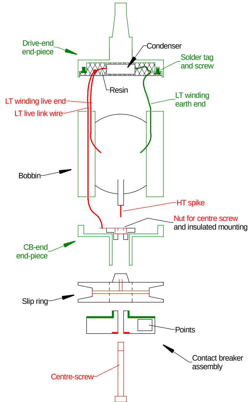
Typical exploded schematic 'BEFORE'
