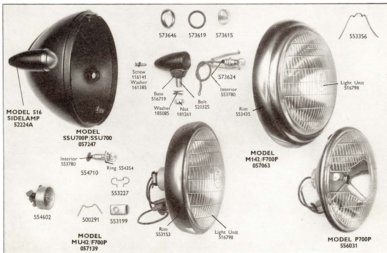
M142/F700P. 8" diameter rim. Ordering No. 057063.
